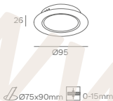
Surface frame TC-0084
